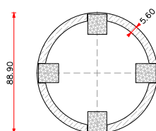
Cross cut pipe (A-A')
