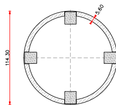
Cross cut pipe (A-A')
