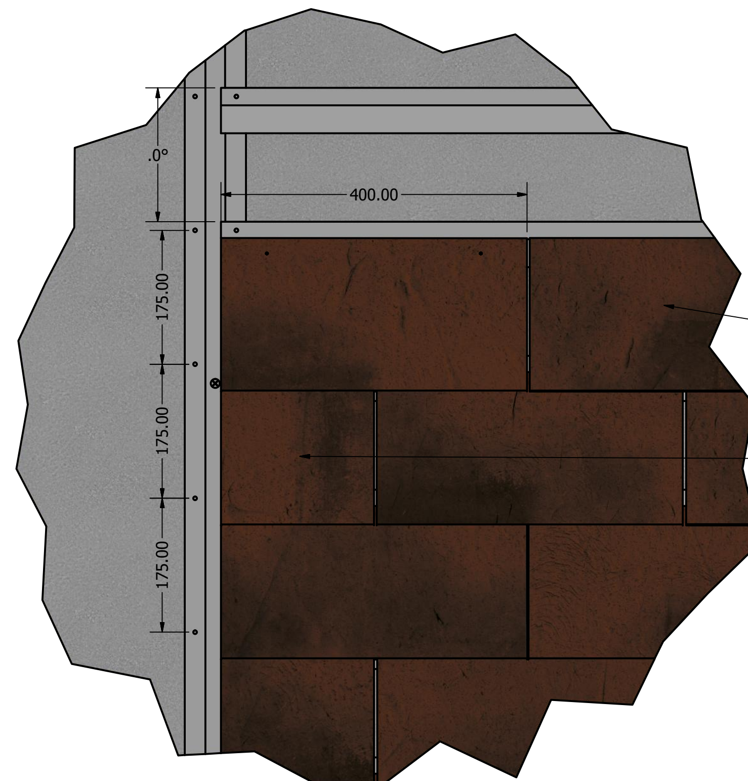
DETAIL B SCALE 1 / 5
