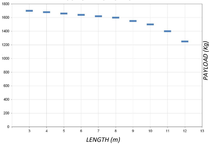
P40 SINGLE MAST LOAD CHART
