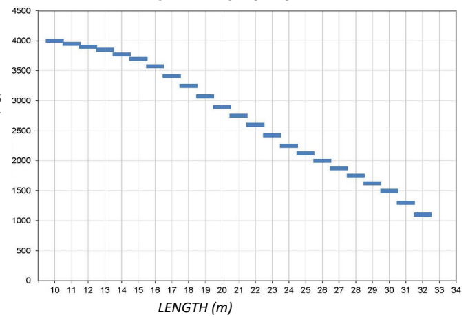
P40 TWIN MAST LOAD CHART
