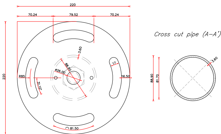
Part 1 – Top view flange
