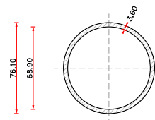
Cross cut pipe (A-A')
