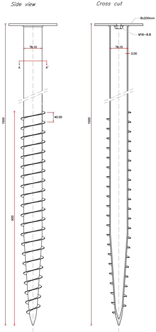
Cross cut pipe (A-A')
