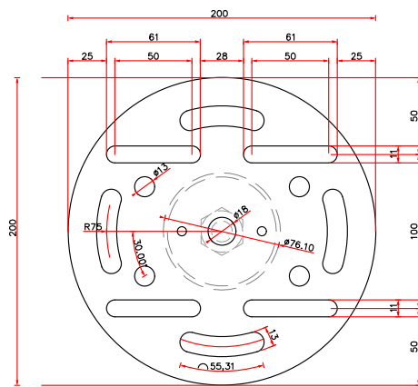
Top view flange
