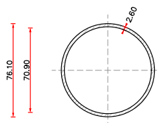
Cross cut pipe (A-A')
