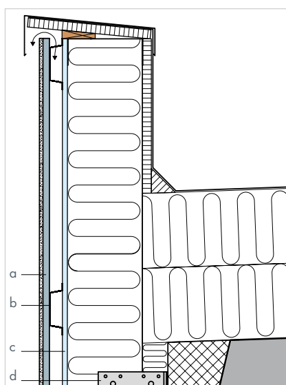
YP10: Murkrone
