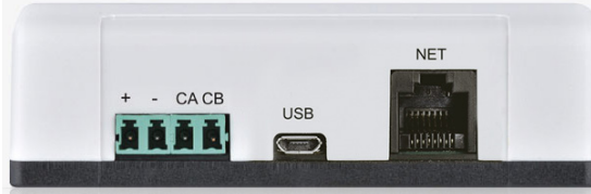
STRØMFORSYNING Strømforsyning 12Vdc 10W TCP-IP (standalone) | JA320410
